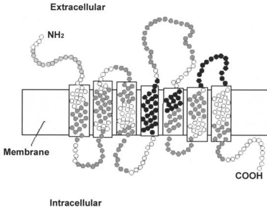
Figure 3. Structure of olfactory cell-surface receptor molecules. Greyshade relates to degree of variability among OR genes, probably related to odorant binding properties. From Weiss and Buchanan. 2
