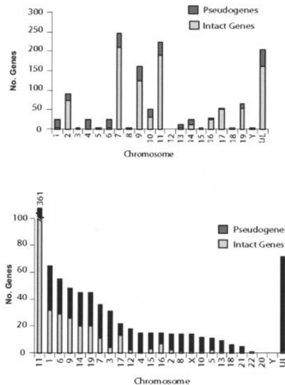
Figure 4. Distribution of olfactory receptor genes and the fraction of these that are pseudogenes, in the mouse (top) and human (bottom) genomes. From Weiss and Buchanan. 2
