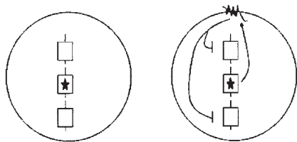
Figure 5. Hypothetical means to achieve single olfactory receptor gene expression in an olfactory neuron. The OR protein coded by lucky first gene to be expressed in a given ON (star) makes its way to the cell surface (arrow) but somehow also back to the nucleus where it inhibits expression of other ORs (feedback lines). 8
