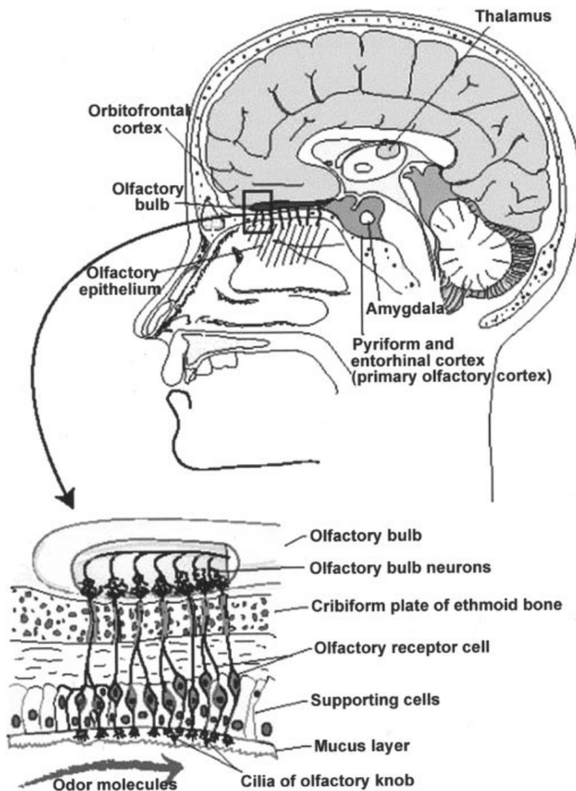
Figure 2. The olfactory detection apparatus. From Weiss and Buchanan. 2
