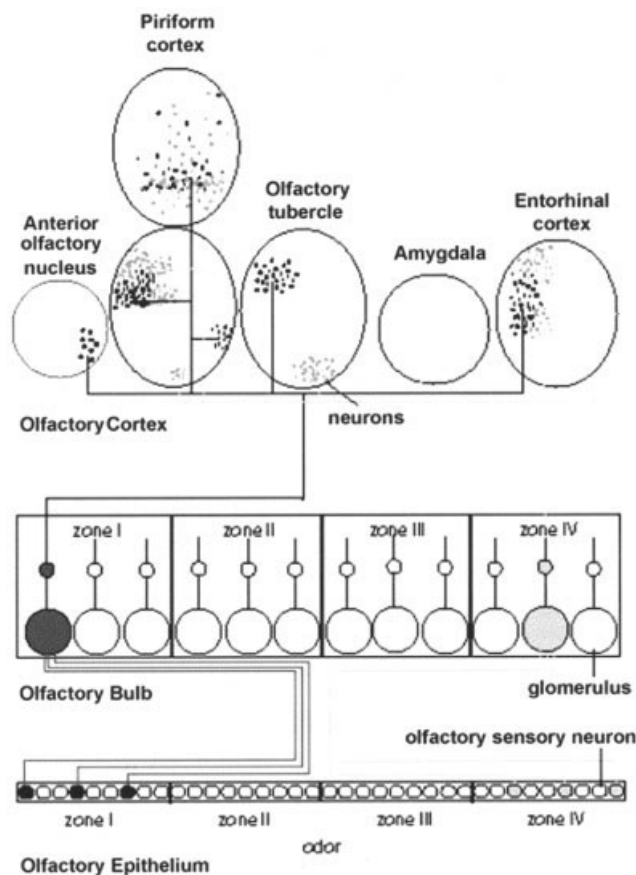
Figure 6. Orderly olfactory wiring from the OR in the olfactory epithelium, to glomeruli in the olfactory bulb to various olfactory regions in the brain. From Weiss and Buchanan. 2
